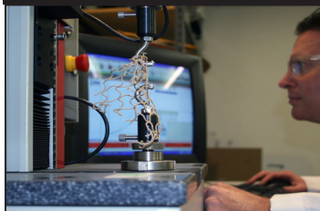
Actual ISO 1806 testing procedure at our manufacturing plant in CA.
